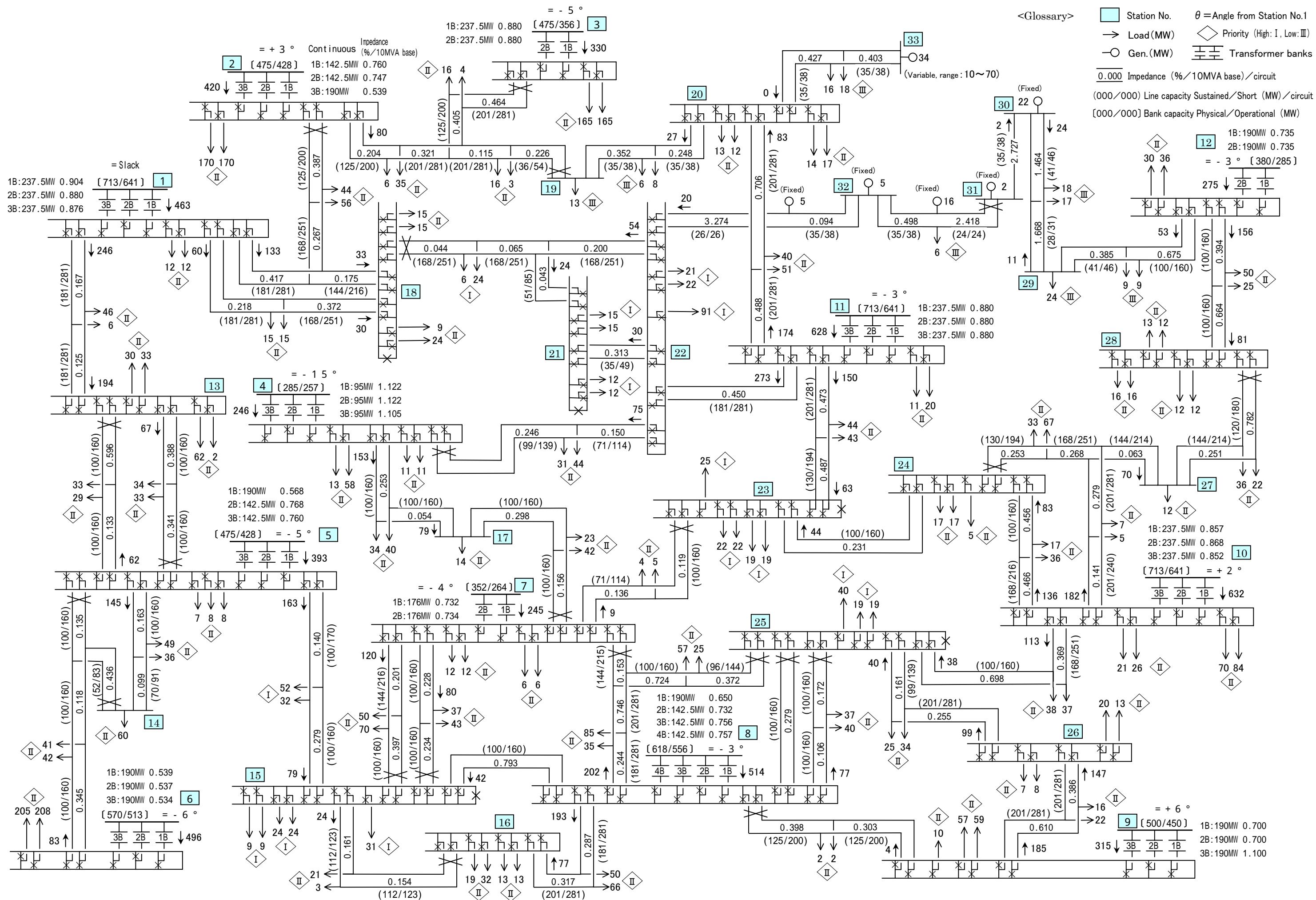
Fig. 2.1 : 77kV Provincial system model (Normal load)
