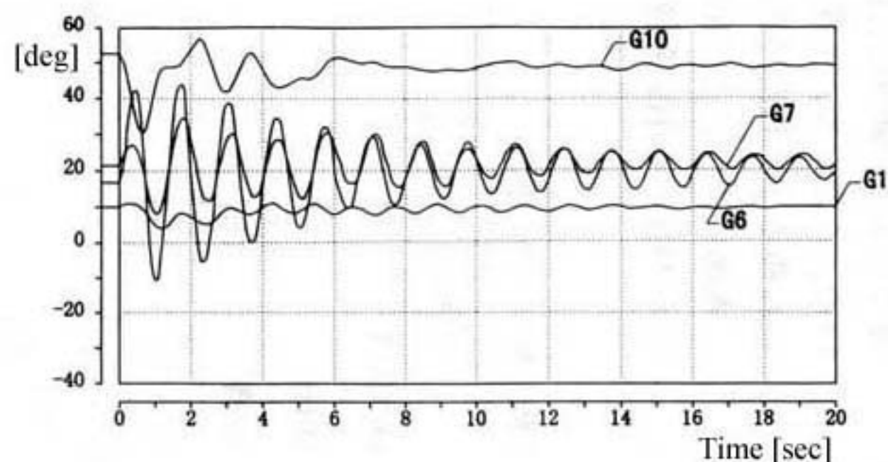
(b) The Excitation System of the G6 is changed to LAT = 2 (Thyristor Exciter Model)
