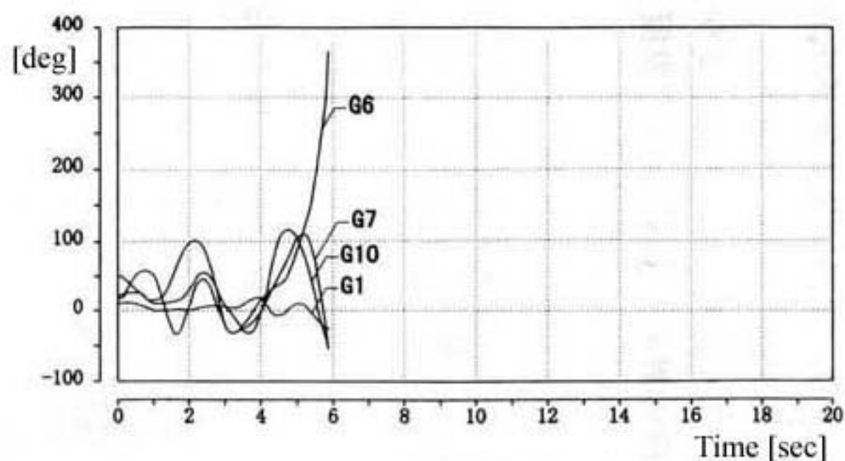
(a) LAT = 1 (Rotating Exciter Model) (Base Case)
