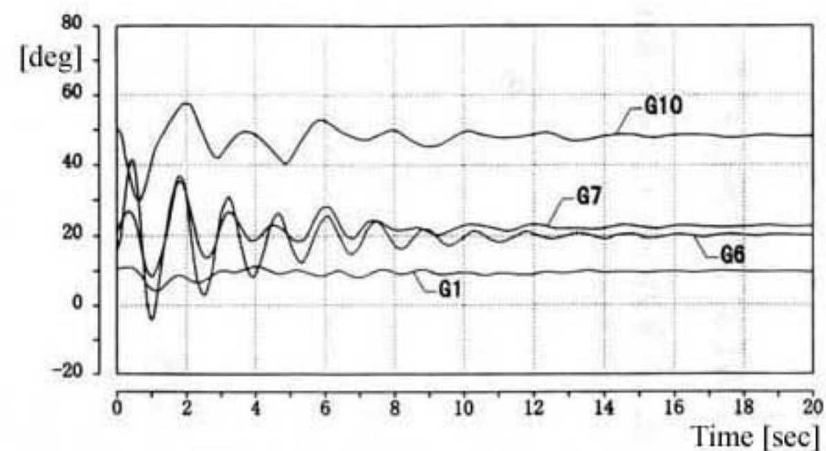
(c) The Excitation System of the G6 is changed to LAT = 102 (Thyristor Exciter + PSS)
