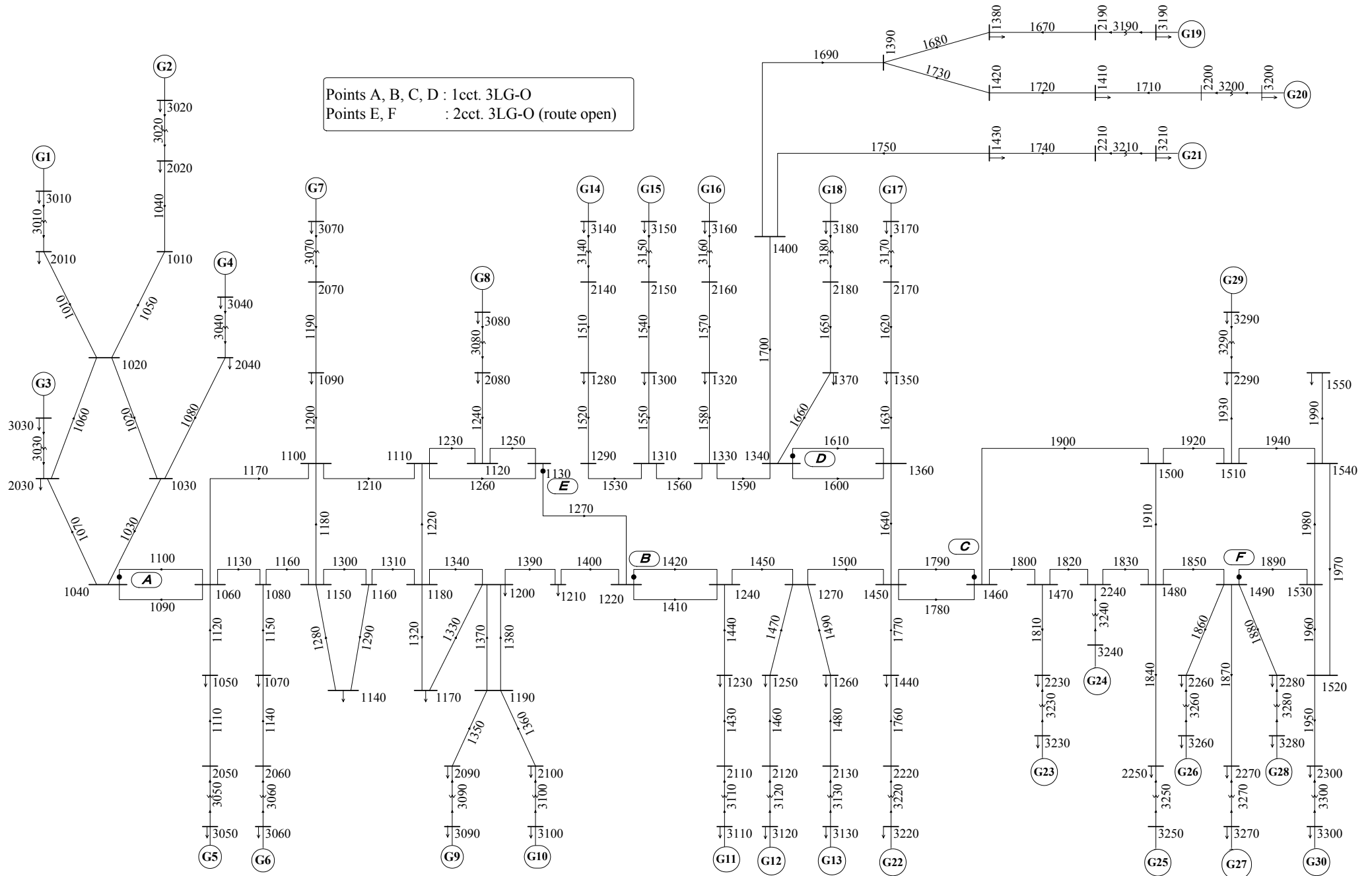
Fig.5.1 IEEJ WEST 30-machine System Model (Node No., Branch No., Disturbance Points)
