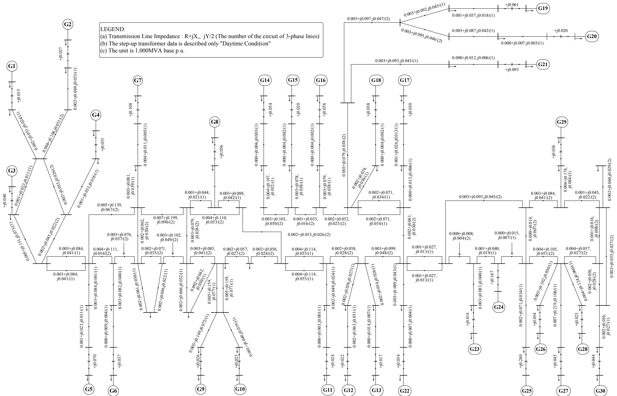
Fig.5.2 IEEJ WEST 30-machine System Model (Impedance Map)
