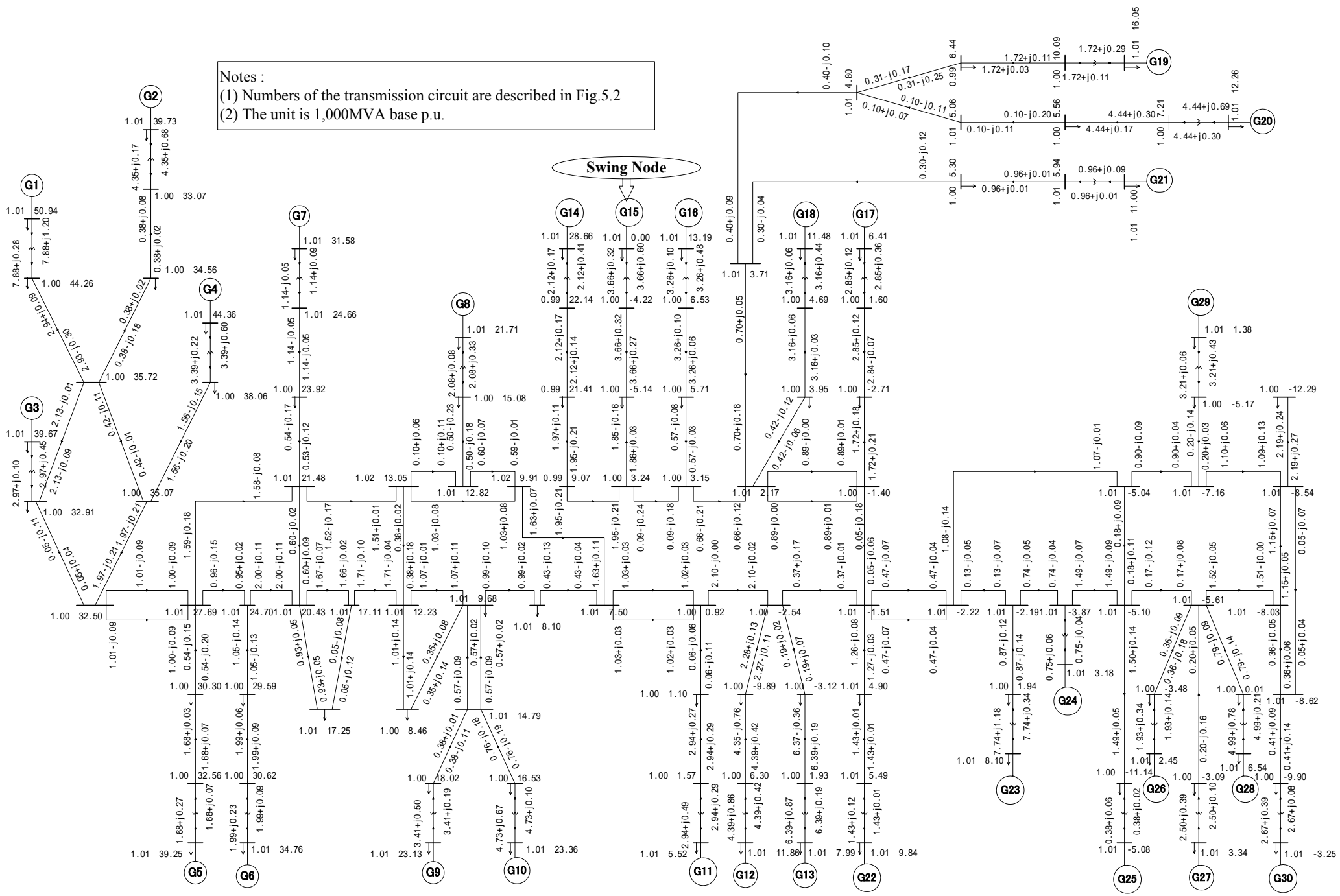
Fig.5.3(a) IEEJ WEST 30-machine System Model (Load Flow Map, Daytime Condition)
