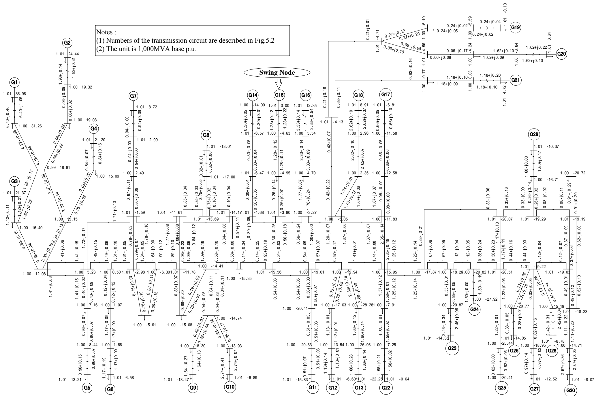
Fig.5.3(b) IEEJ WEST 30-machine System Model (Load Flow Map, Nighttime Condition)
