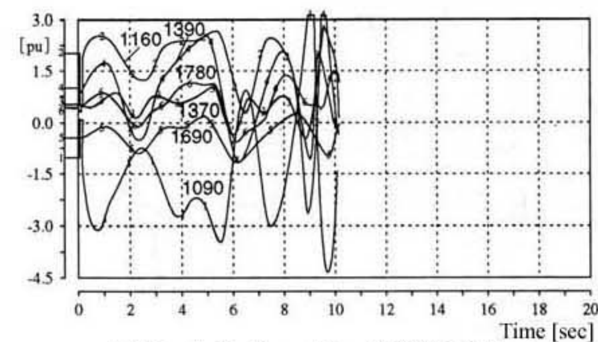
(c) Line Active Power Flow (1,000 MVA Base)
