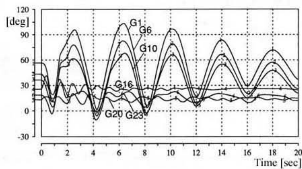
(a) Generator Internal Angle (G15 Base)
