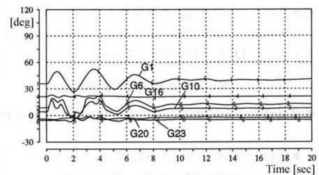
(a) Generator Internal Angle (G15 Base)
