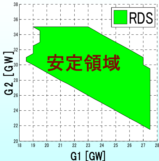
PV予測誤差:0%
